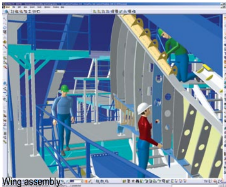
Wing assembly
